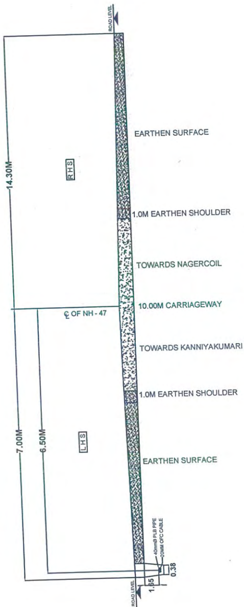
CROSS SECTION AT Km: 640/300
