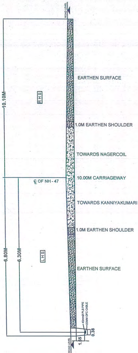
CROSS SECTION AT Km: 641/100
