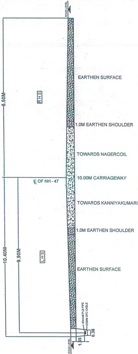
CROSS SECTION AT Km: 641/700
