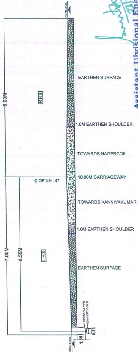
CROSS SECTION AT Km: 641/400
