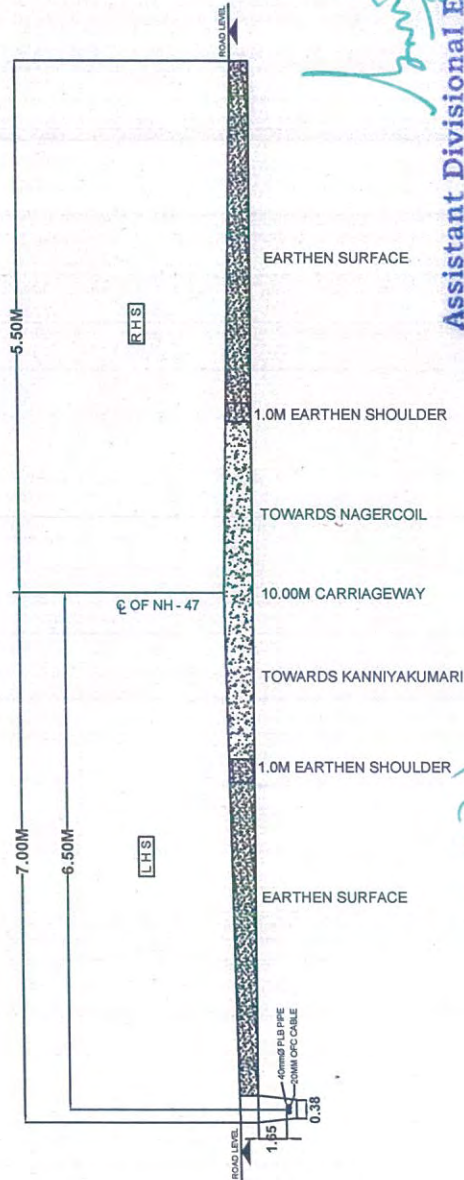
CROSS SECTION AT Km: 641/600
