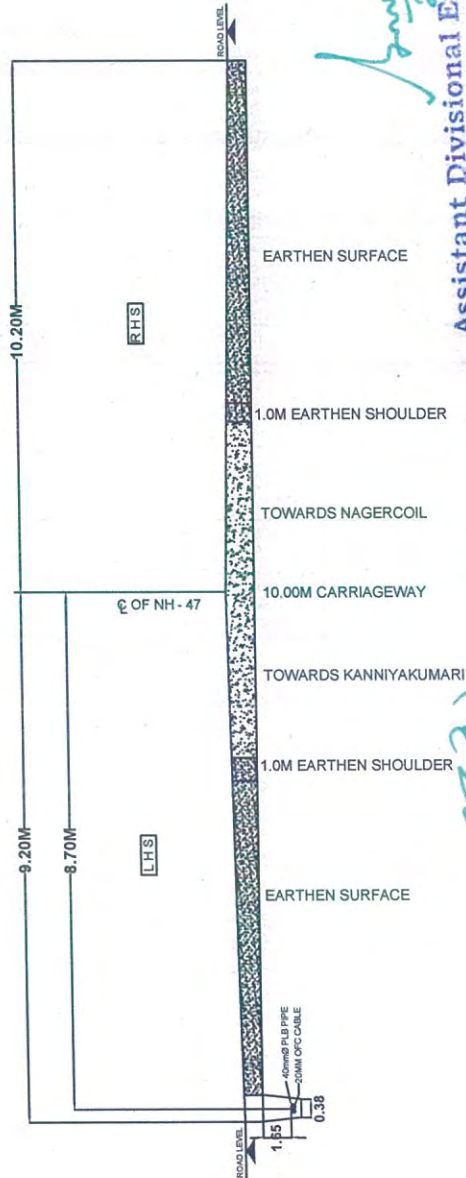
CROSS SECTION AT Km: 640/800
