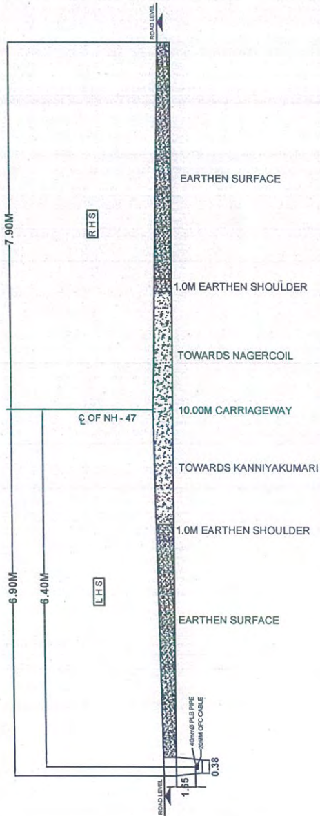
CROSS SECTION AT Km: 641/500
