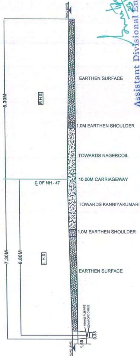
CROSS SECTION AT Km: 641/200
