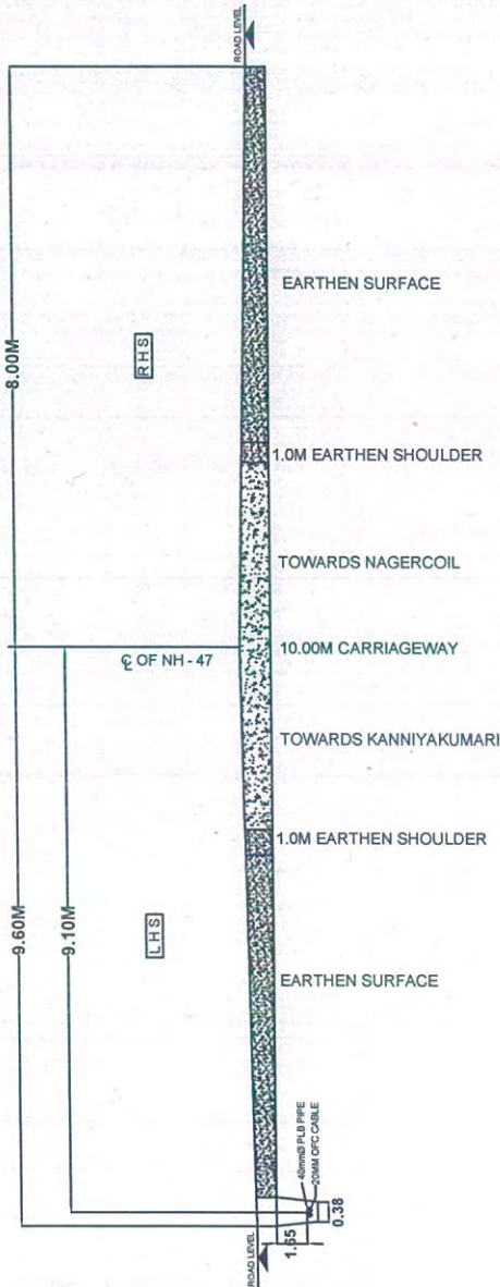
CROSS SECTION AT Km: 641/300
