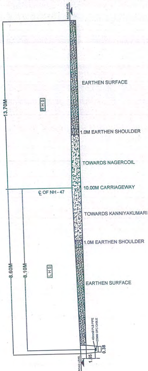
CROSS SECTION AT Km: 640/100
