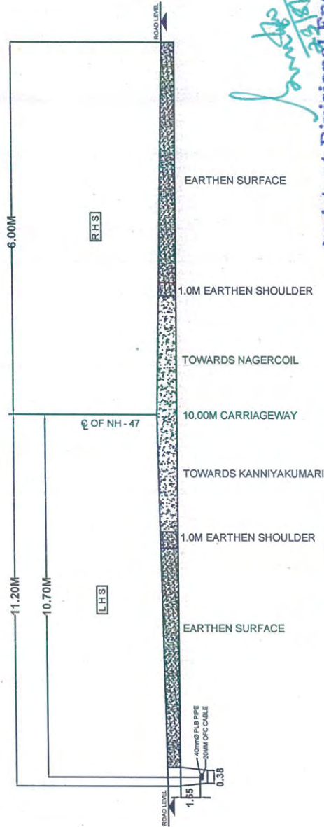
CROSS SECTION AT Km: 641/800 & Km: 641/830
