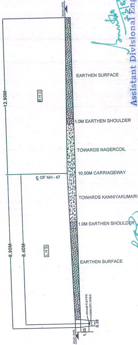
CROSS SECTION AT Km: 640/200
