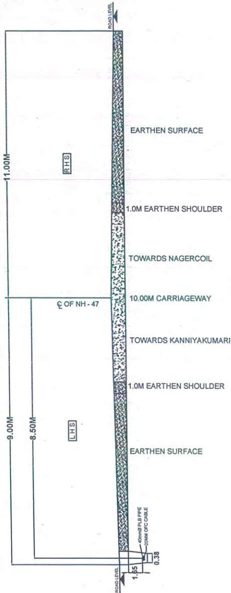
CROSS SECTION AT Km: 640/900
