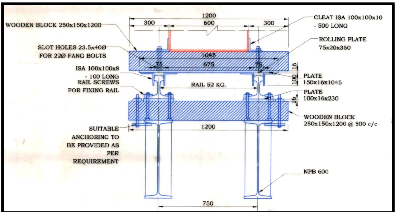
Fig 11: Typical section of Skidding Arrangement
