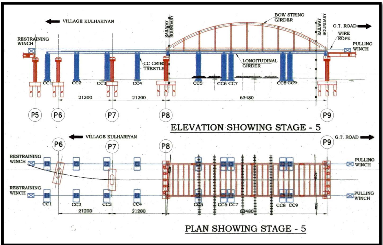
Fig 10: Elevation and Plan of Launching Stage-5
