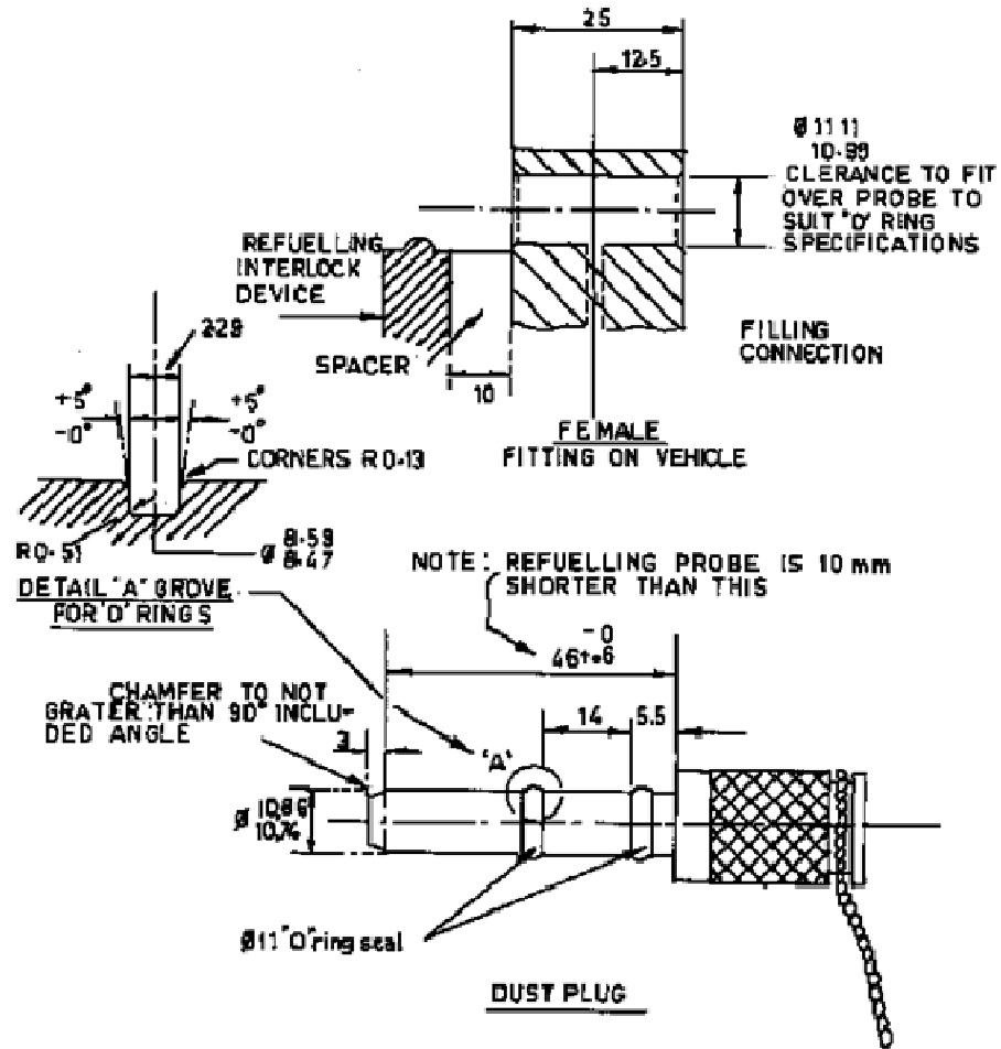
DUST PLUG CNG VEHICLE FILLING SYSTEM
