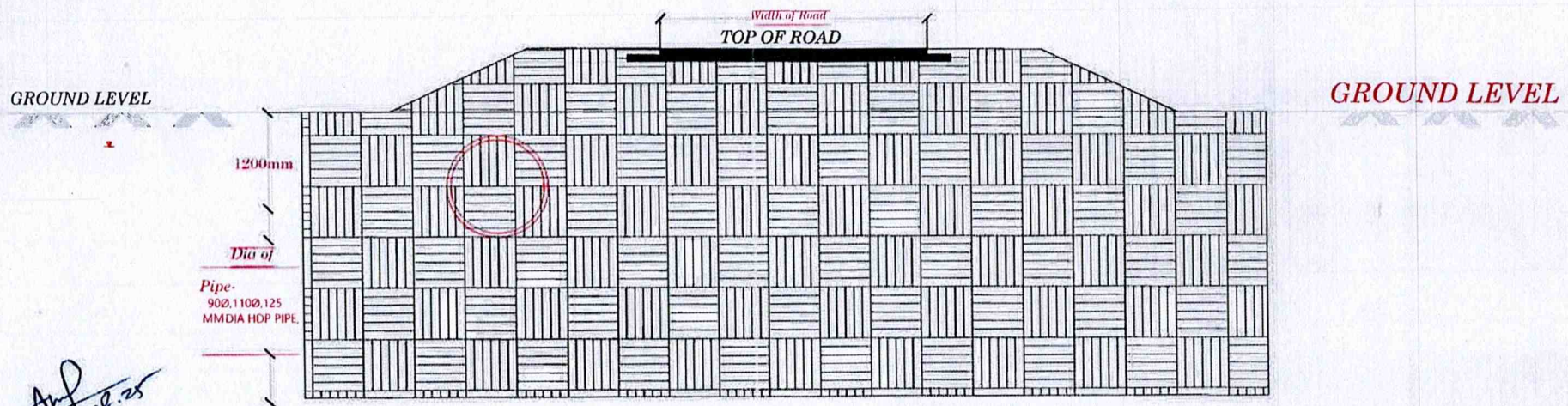
TYPICAL CROSS SECYION SHOWING PIPE ALNOG THE ROAD
