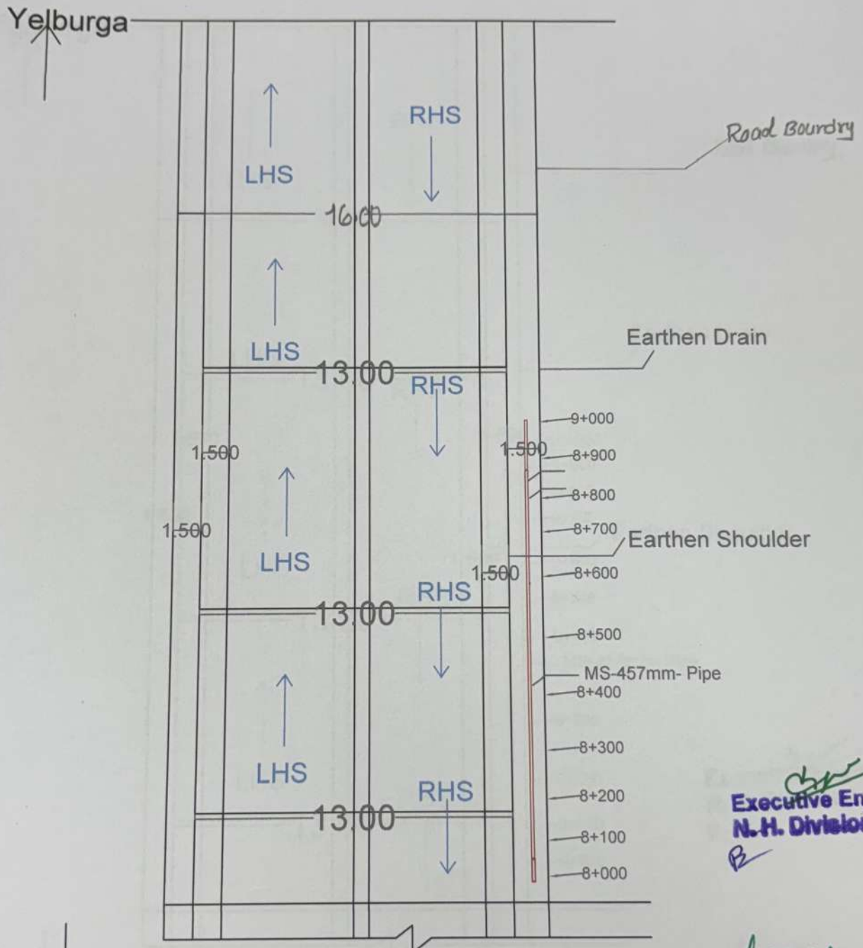
STRIP PLAN
