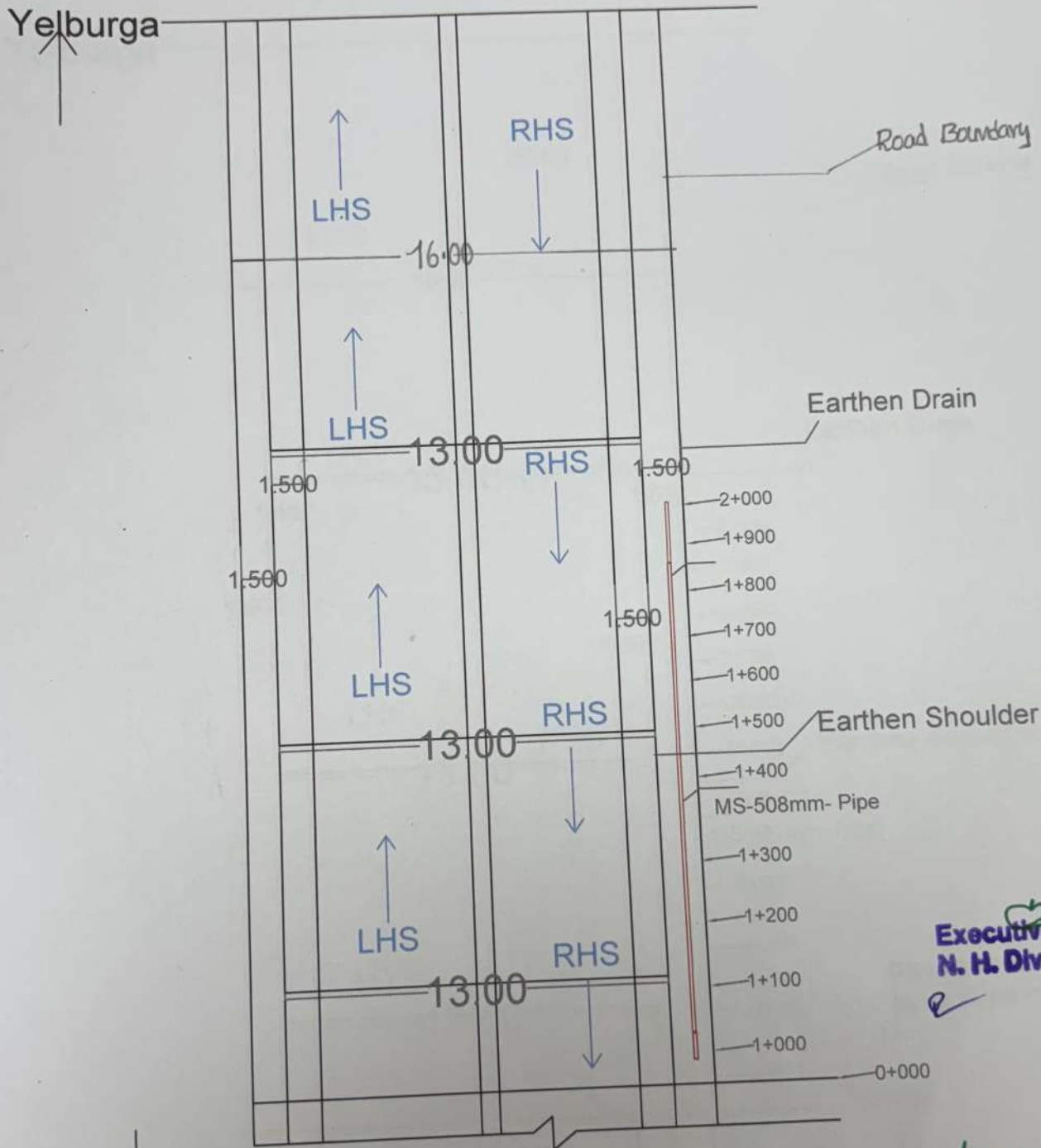
STRIP PLAN
