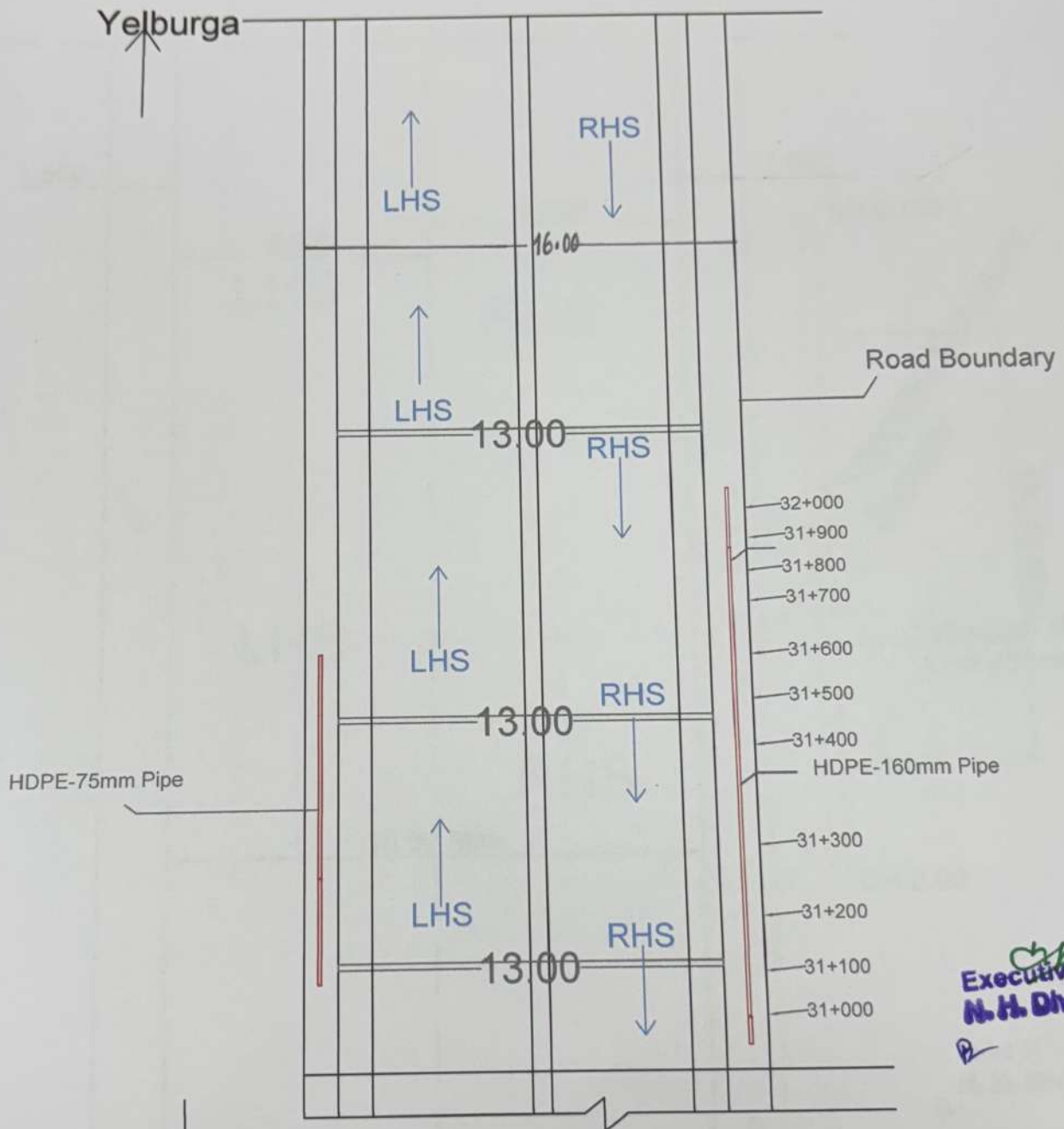
STRIP PLAN
