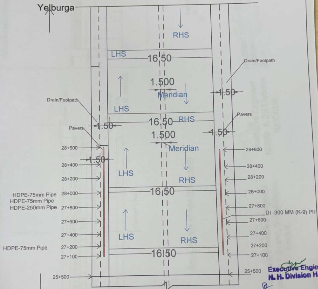
STRIP PLAN
