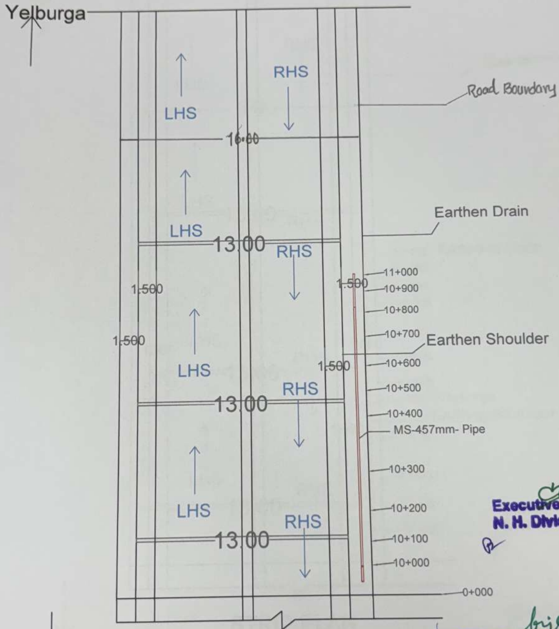
STRIP PLAN
